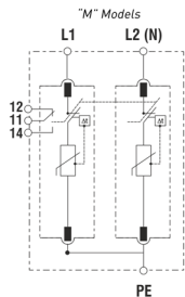
IT (1Ph+N) - 2PG
