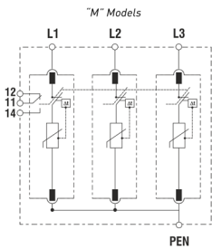
TNC (3Ph) - 3PG
