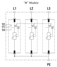
IT (3Ph) - 3PG
