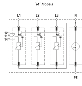
TT (3Ph+N) - 4PG
