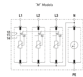
TT (3Ph+N) - 4PG
