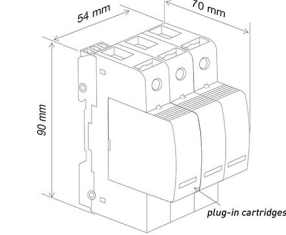
3 Poles
