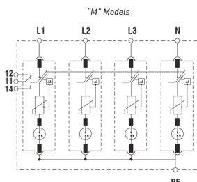
TNS LF (3Ph+N) - 4P
