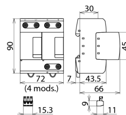
Dimension drawing DV M TN 255 FM
