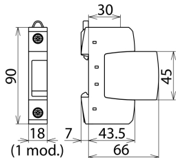
Dimension drawing DG S ...
