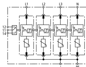
Basic circuit diagram DG M TNS ... FM
