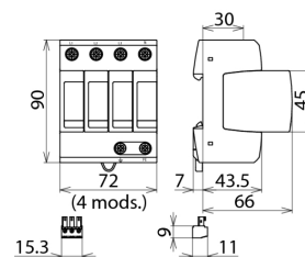
Dimension drawing DG M TNS ... FM
