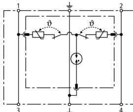
Basic circuit diagram DR M 2P ...
