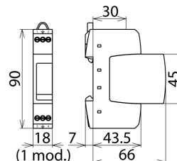
Dimension drawing DR M 2P ...
