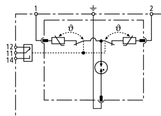
Basic circuit diagram DR M 2P ... FM
