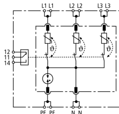
Basic circuit diagram DR M 4P ... FM
