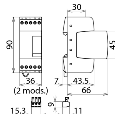
Dimension drawing DR M 4P ... FM
