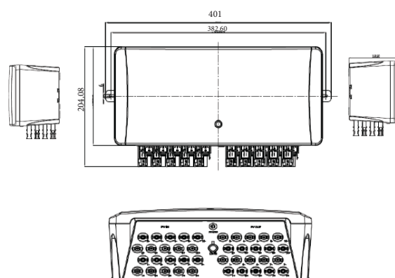
Strings: 10
